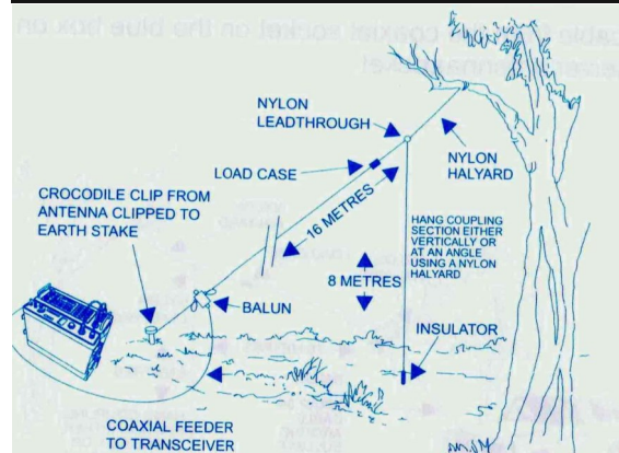
As an emergency antenna, the SWE-100 can be deployed in several configurations
